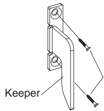
#8 x 1-1/4" PH FH HD SM SS Screw (2) Part # 017806
