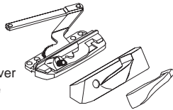
Right Dyad Operator with Left Operator Cover and Handle Package
