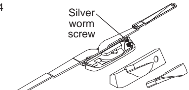
Left Dual Arm Operator with Left Operator Cover and handle Package
